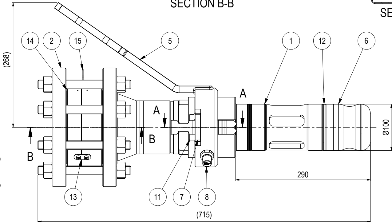
SECTION B-B
