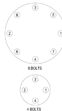
Figure 8 - Bolt Tightening Sequence
